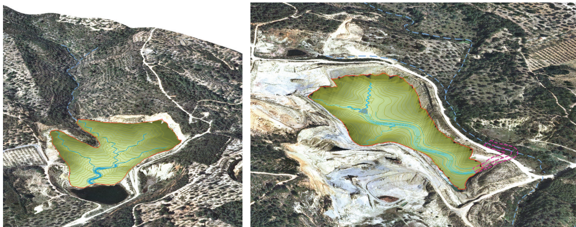
Figure 10. Left, proposed GeoFluv solution for the Aurora quarry (7.3 hectares, 18 acres); as it can be seen, the designed area hydrologically connects a stream with an existing pond (dark area). Right, the Pastor quarry pit has been designed to play the role of a natural “storm surge basin” of a watershed with an area of 279 ha (689 acres); the dashed pink line represents the bypass from the Rocacorba stream to the pit. The main contribution of this design is that the “storm surge basin” will be a natural landscape, restoring 24 ha (59 acres). In addition to the explained solutions, in both cases the geomorphic reclamation will be the basis for restoring valuable and threatened habitats.
