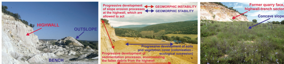
Figure 2. Left (January 1995), main landforms created by the exploitation of La Revilla quarry. Center (February 1995) — the landform design proposed two different zones for managing surface slope processes; the image shows them immediately after they were built. The right picture (May 2006) shows the landscape evolution at the two referred zones; the accommodation of fallen debris at the trench and the geomorphic stability at the concave slope can be clearly seen. All the details about the geomorphic design, cut and fill balance, and other relevant information are explained at Martín Duque et al. (1998).
